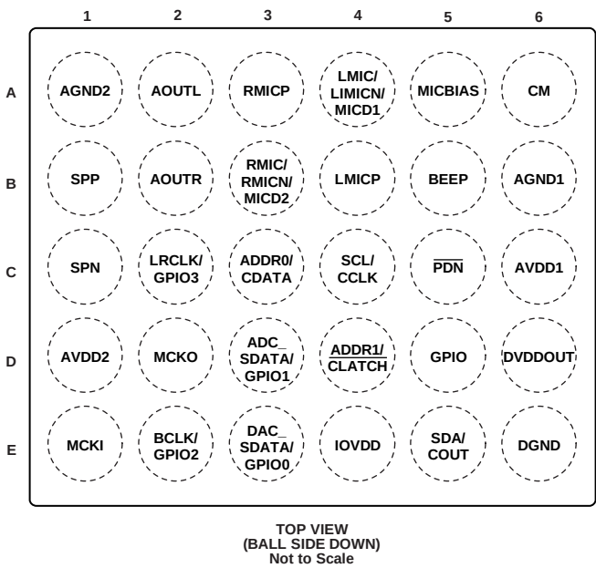
Figure 8. 30-Ball, 6 × 5 WLCSP Pin Configuration (Bottom View)
