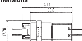
Panel/Free-Hanging Type
