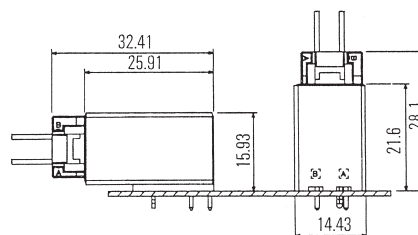
Horizontal/Vertical Type
