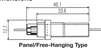
Panel/Free-Hanging Type
