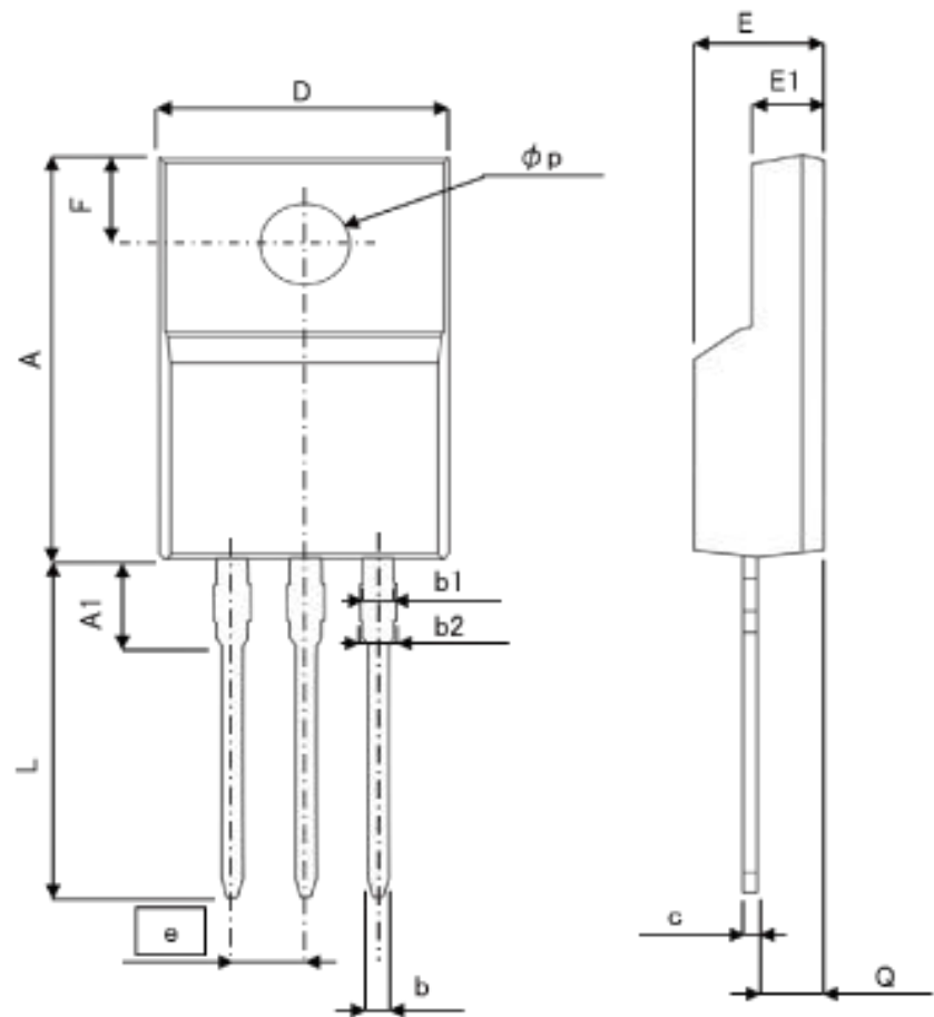
TO-220FM
