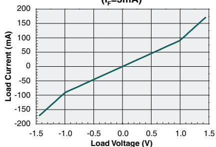
Typical Load Voltage vs. Load Current ( I_F=5\text{mA} )
