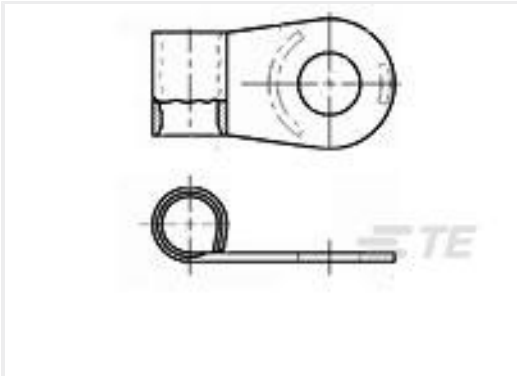
TE Part #36271 TERMINAL,SOLIS FLAG R 12-10 10
