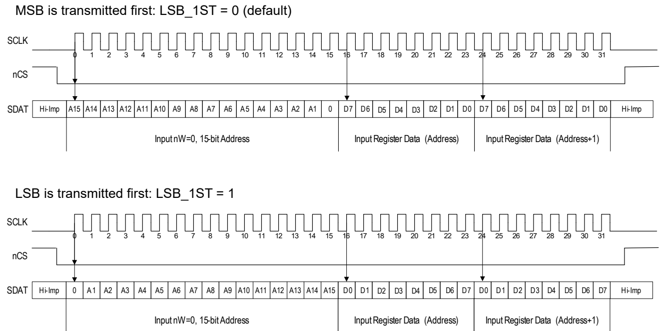
Figure 16. Logic Diagram: SPI 3/4-wire WRITE Data into Registers
