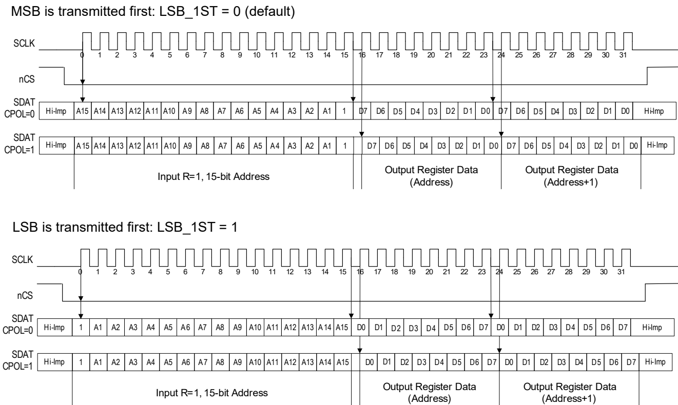
Figure 15. Logic Diagram: SPI 3-wire READ Data from Registers for CPOL = 0 and CPOL = 1
