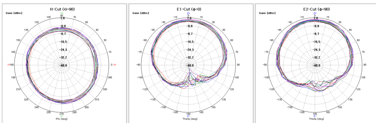
Figure 6: Radiation pattern at the L2/L5/E5 band. The 2-D cuts are measured at 1166 - 1249 MHz.
