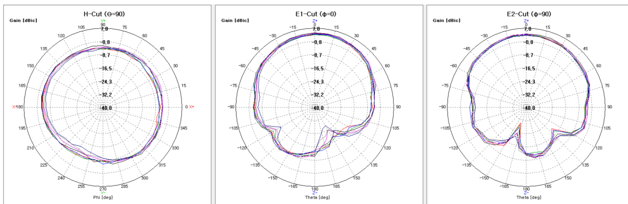
Figure 5: Radiation pattern at the L1 band. The 2-D cuts are measured at 1559 - 1606 MHz.
