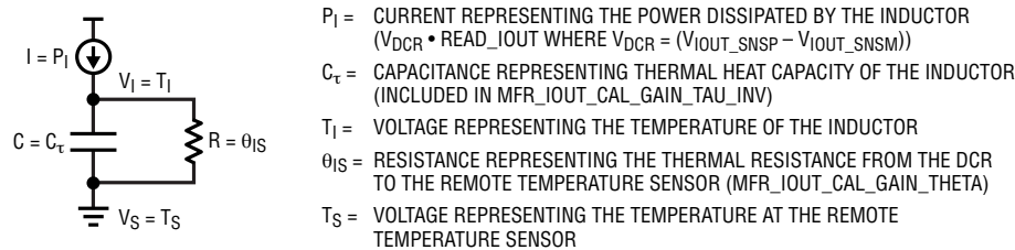
Figure 19. Electronic Analogy for Inductor Temperature Model
