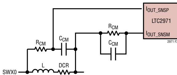
Figure 34. DCR Current Sensing Circuits
