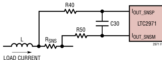
Figure 33. Sense Resistor Current Sensing Circuits
