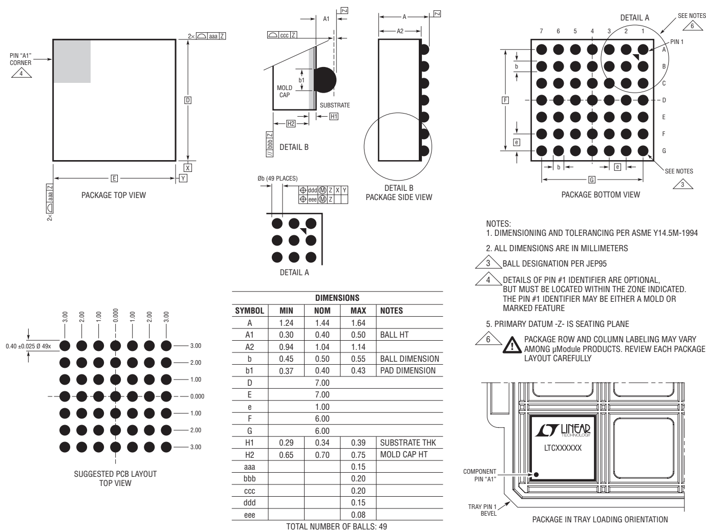
BGA Package 49-Lead (7.00mm × 7.00mm × 1.44mm) (Reference LTC DWG # 05-08-1615 Rev 0)
