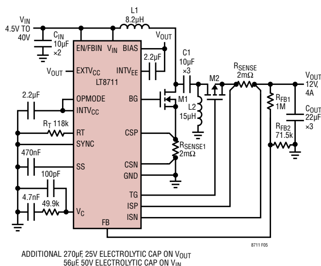
Figure 5. SEPIC Converter—The Component Values Given Are Typical Values for a 200kHz, 4.5V–40V to 12V/4A SEPIC
