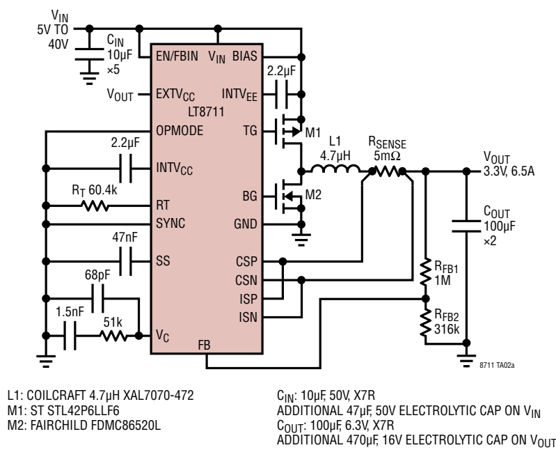
400kHz, 5V–40V Input to 3.3V/6.5A Buck
