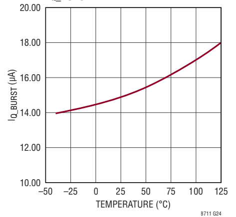
I Q_BURST vs Temperature
