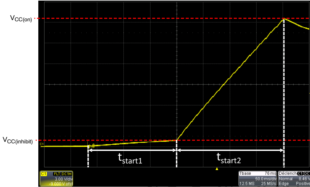
Figure 45. V_{\text{CC}} at Start-up is made of Two Segments given the Short-circuit Protection Implemented on the HV Source
