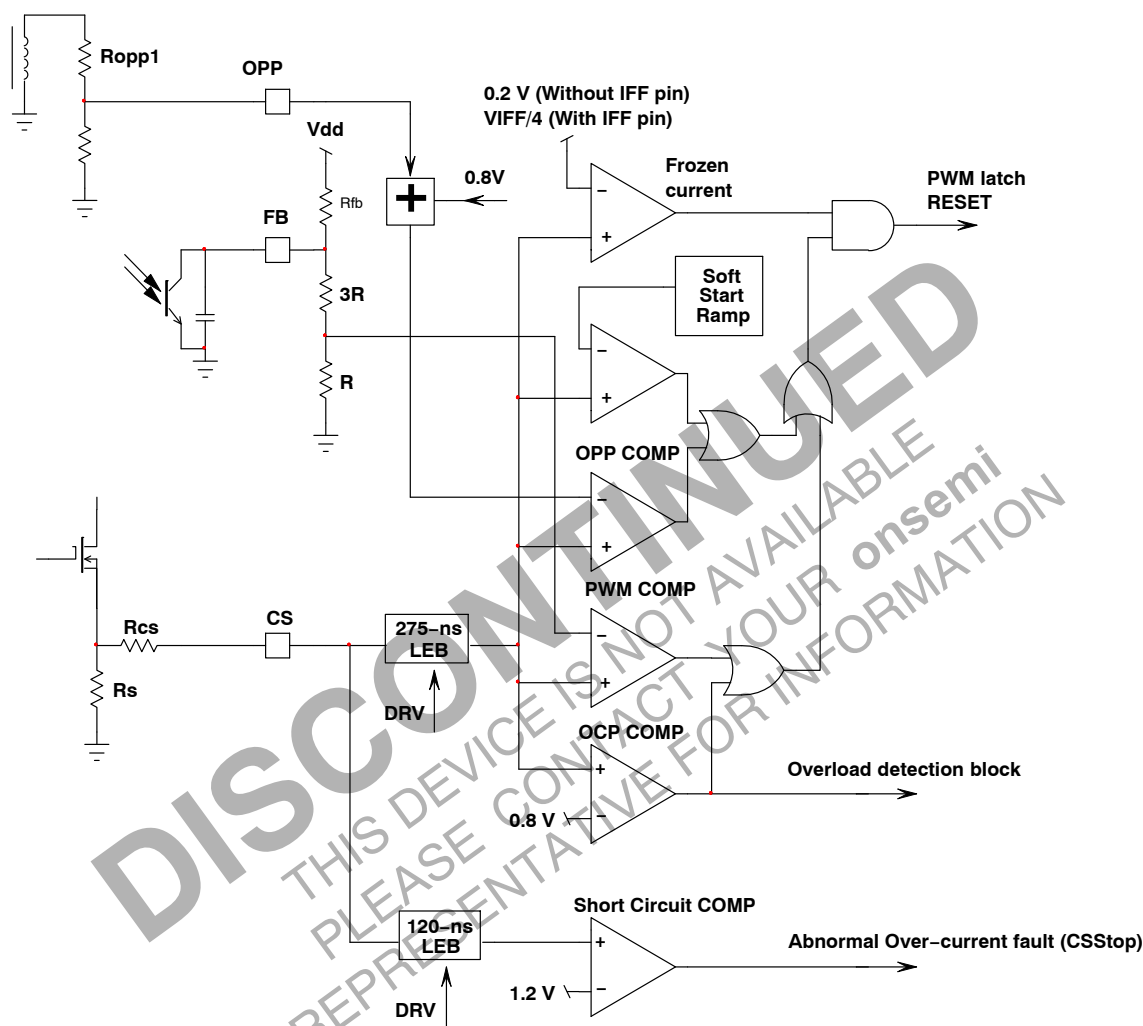
Figure 56. Current Setpoint
