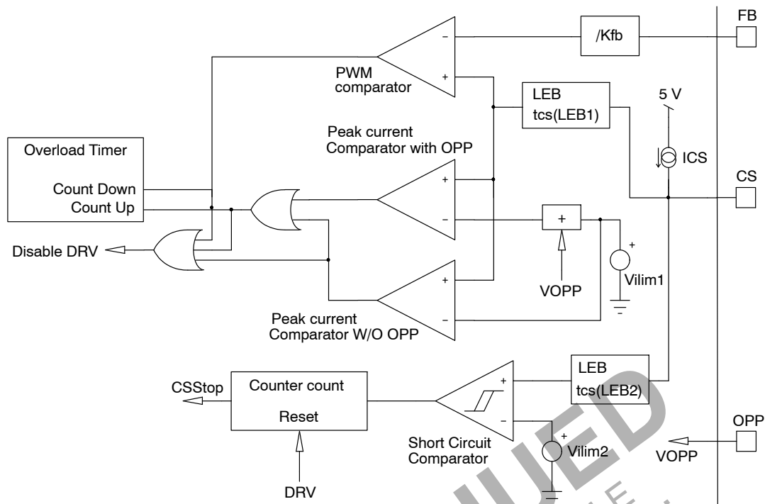
Figure 57. Overload Circuitry
