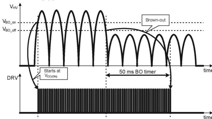
Figure 47. Internal Circuit Implements a 50-ms Timeout to Accommodate with Full-wave Rectification
