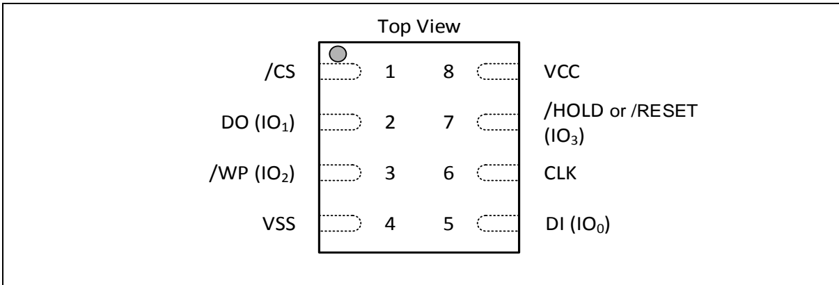
Figure 1b. W25Q16RV Pad Assignments, 8-pad WSON 6x5-mm, USON 2X3-mm (Package Code CP, XH, UU)
