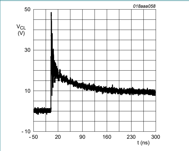
Fig. 8. Clamped +8 kV pulse waveform (IEC 61000-4-2 network)
