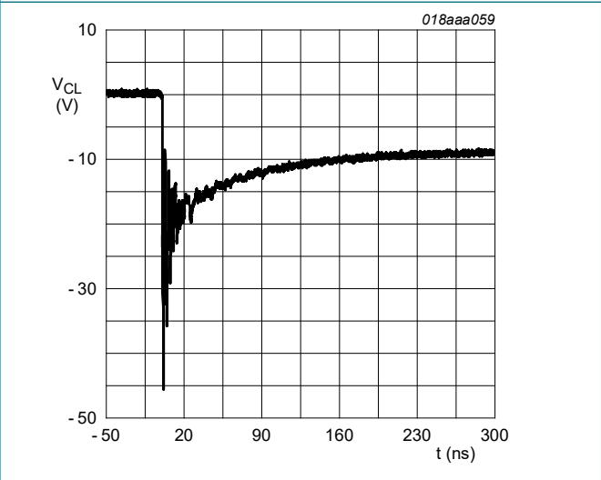
Fig. 9. Clamped -8 kV pulse waveform (IEC 61000-4-2 network)
