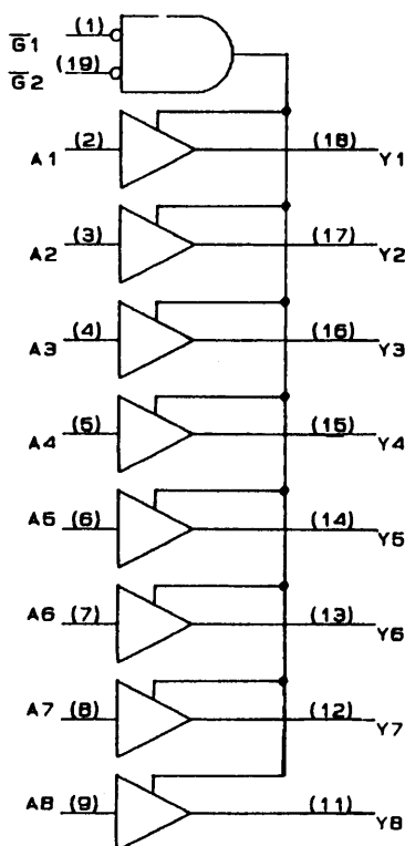
LOGIC DIAGRAM
