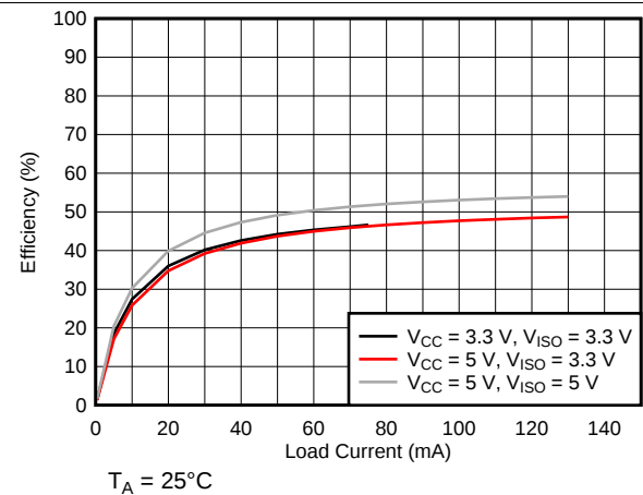
Figure 6. ISOW7841 Efficiency vs Load Current ( I_{ISO} )
