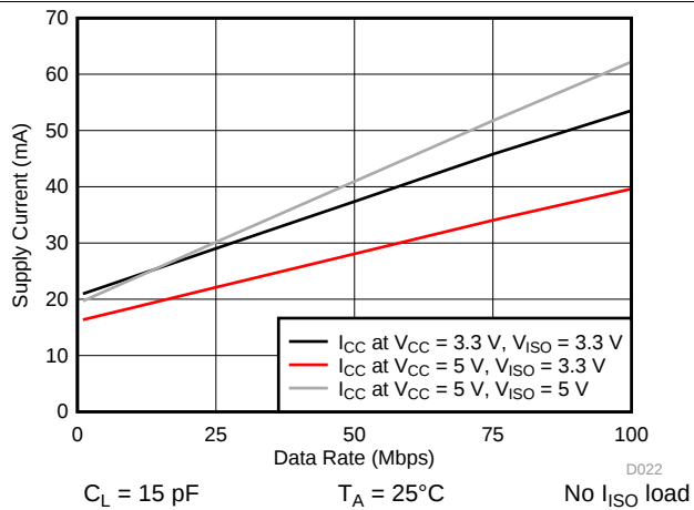
Figure 11. ISOW7840 Supply Current vs Data Rate
