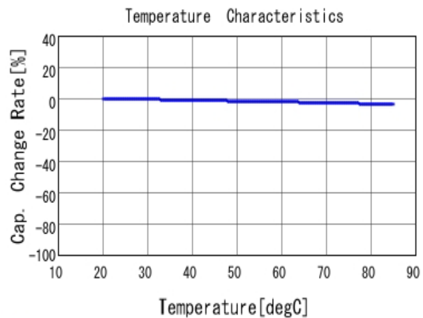
■ DE11XRA220KA4BP01F C-Temp. capchange, DC0V, AC1Vrms
