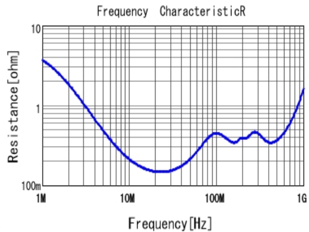
■ DE11XRA220KA4BP01F R DC0V, 20degC
