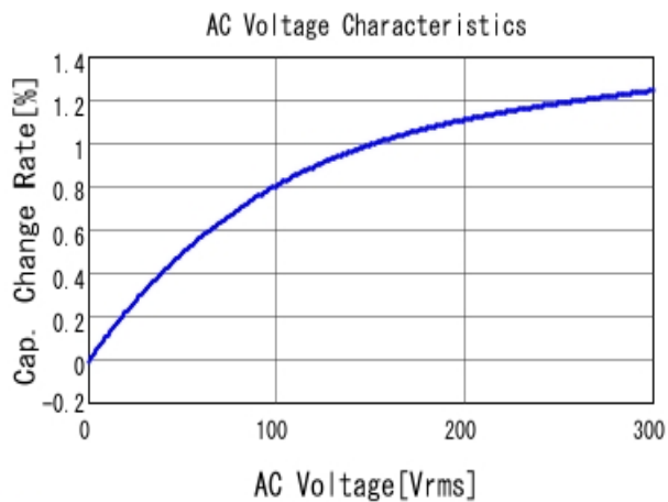
■ DE11XRA220KA4BP01F C-AC Voltage capchange, DC0V, 20.0
