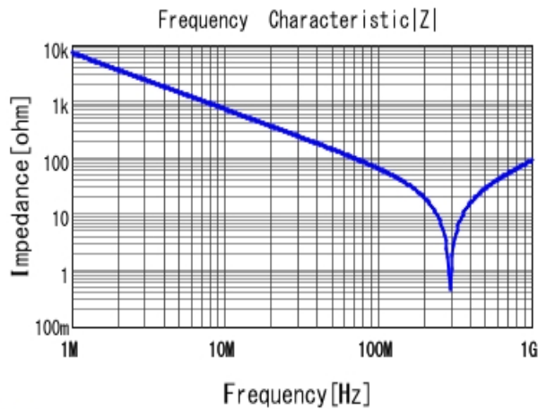
■ DE11XRA220KA4BP01F |Z| DC0V, 20degC
