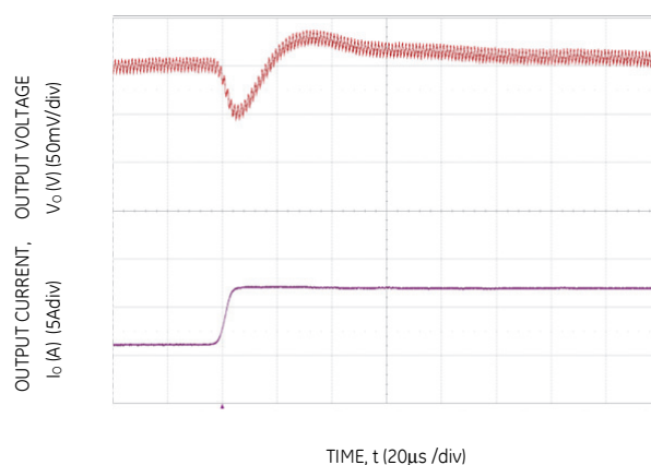
Figure 22. Transient Response to Dynamic Load Change from 50% to 100% at 12Vin, C_{out} = 2 \times 47\mu\text{F} + 1 \times 330\mu\text{F} , C_{Tune}=3300\text{pF} & R_{Tune}=240\Omega
