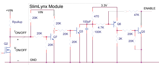
Figure 39. Circuit configuration for using positive On/Off logic.
