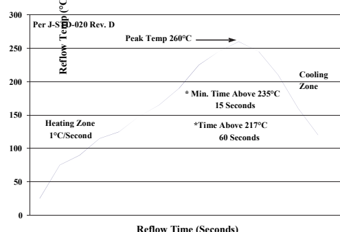
Figure 50. Recommended linear reflow profile using Sn/Ag/Cu solder.
