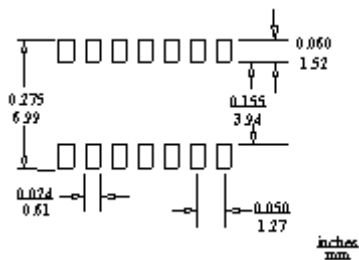
PAD LAYOUT
