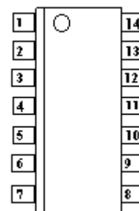
Top Viewing Pin Layout
