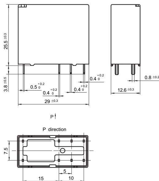
Outline Dimensions
