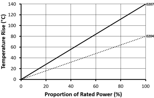
Temperature Rise
