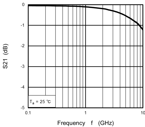
Fig. 8.5 S_{21} - f
