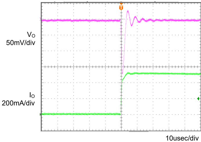
Fig.4 Transient Response (0→0.5A) Co=1 \mu F, Ta=25°C
