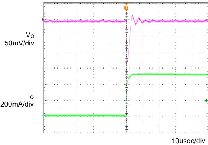
Fig.3 Transient Response (0→0.5A) Co=1 \mu F, Ta=-40°C
