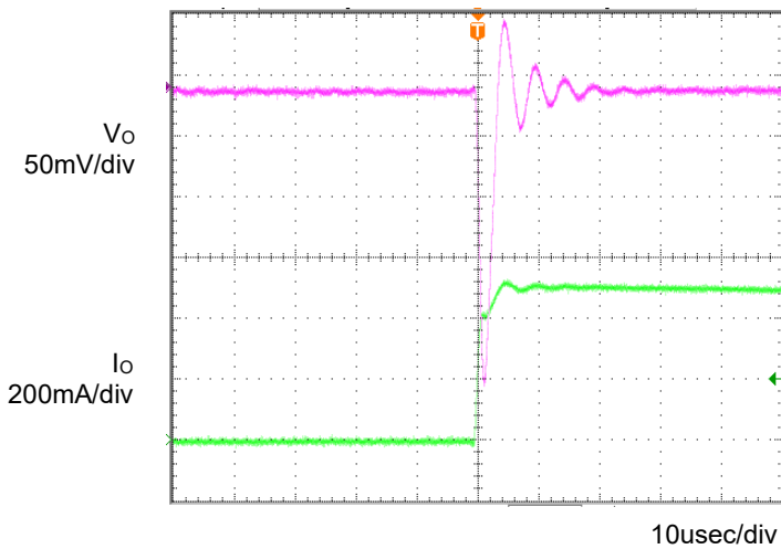
Fig.5 Transient Response (0→0.5A) Co=1 \mu F, Ta=105°C
