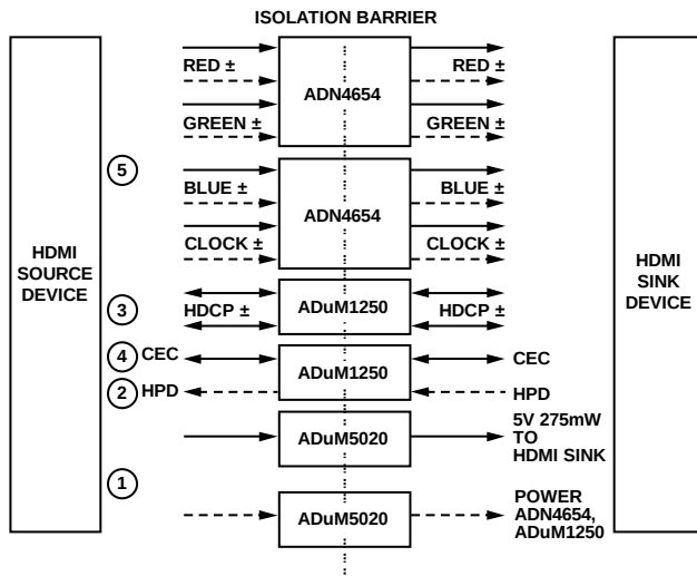
Figure 2. Isolated HDMI Signal Flow Diagram
