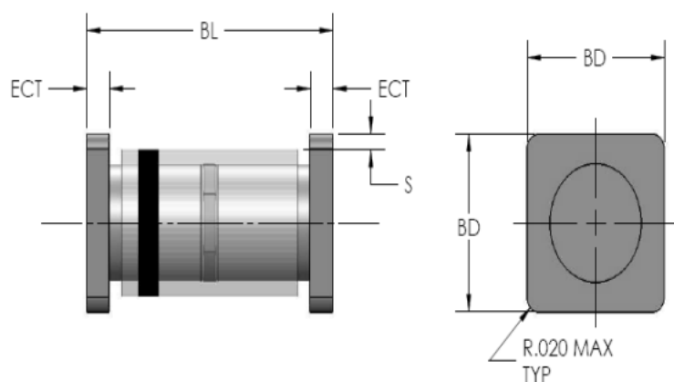
Figure 1: Outline Dimensions
