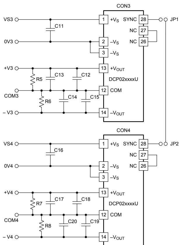
Figure 10-2. PCB Schematic, U Package
