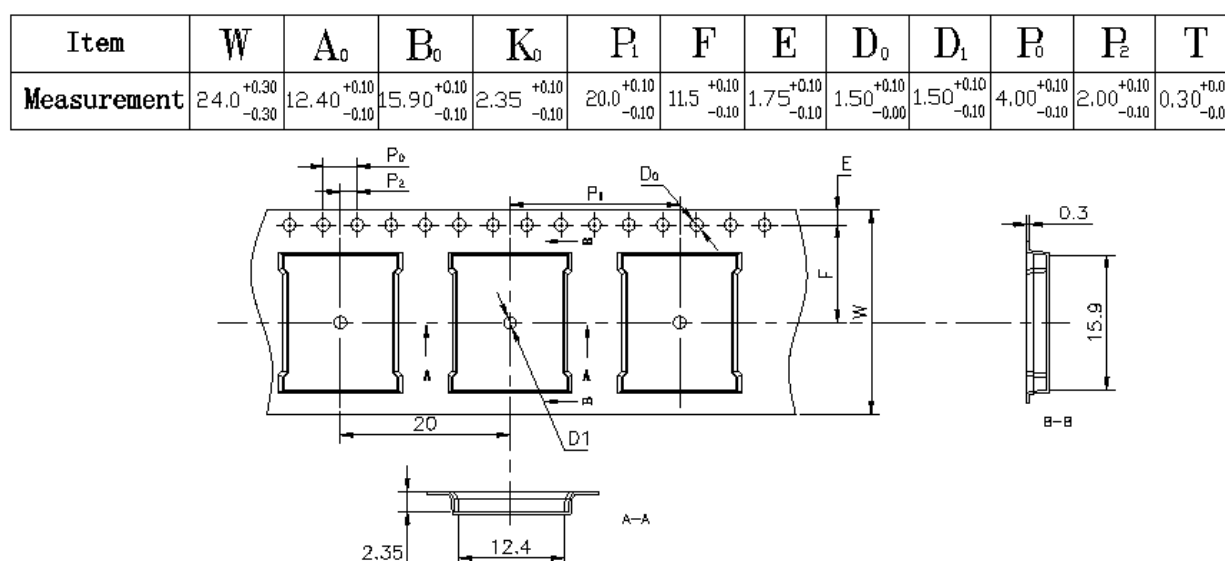
Figure 23. CYBT-343151-02 Tape Dimensions
