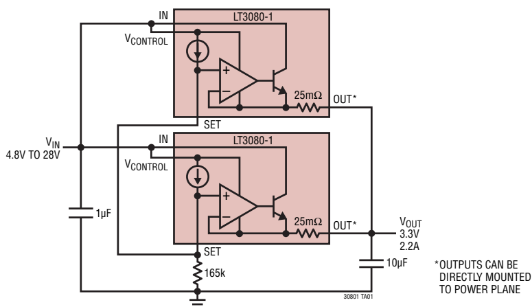
Paralleling Regulators
