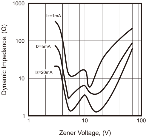
Fig.3 - Effect of Zener Voltage on Impedance
