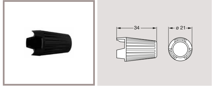
POB.186.GN Spanner for front nut
