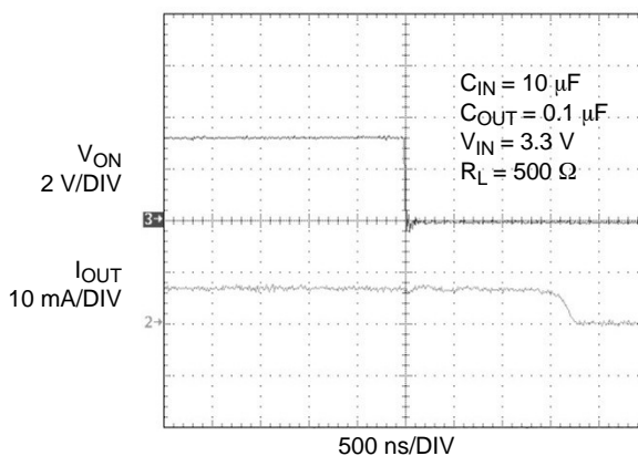
Figure 19. t_{dOFF} Response
