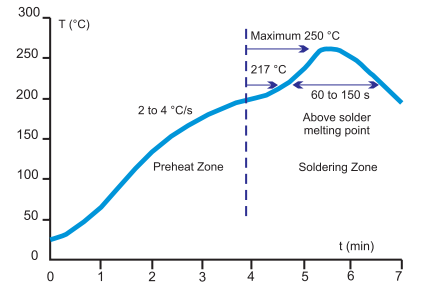
Fig. 3. Reflow Temperature Profile for Pb-free Soldering
