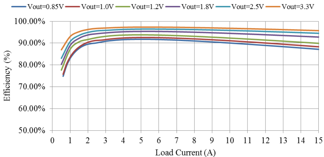
Figure 17. Efficiency vs. Load Current ( V_{in}=5.5\text{ V} )
