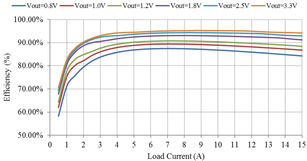
Figure 16. Efficiency vs. Load Current ( V_{in}=12\text{ V} )
