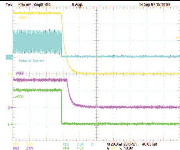
Figure 21. Charger When Adapter Removed
