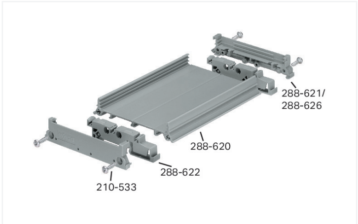
DIN-rail-mount PCB carrier, size 2
