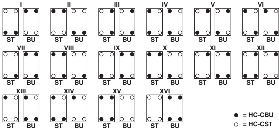
Schematic diagram
