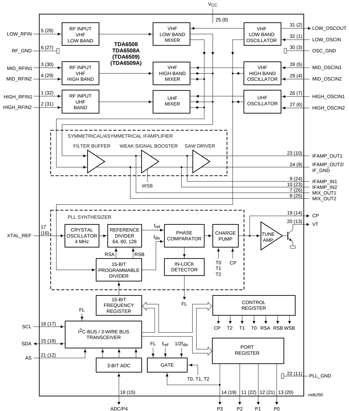
Fig.1 Block diagram.
