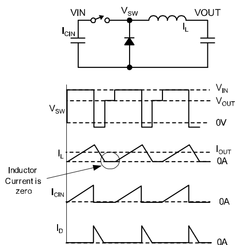
Figure 5. Discontinuous Operation
