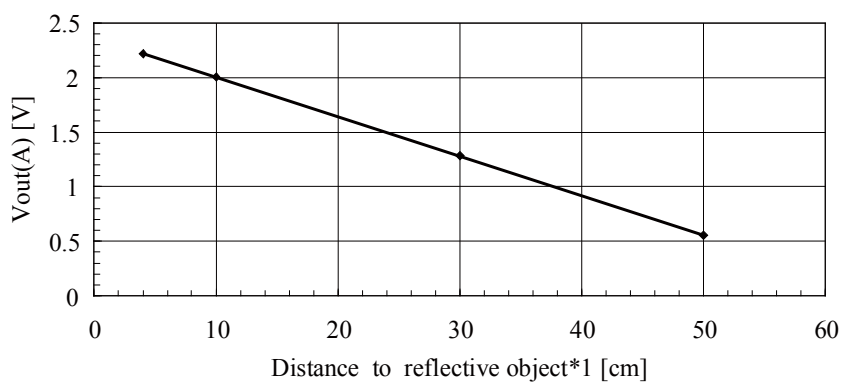
Example of output distance characteristics of GP2Y0E03
