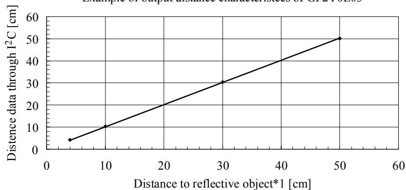
Example of output distance characteristics of GP2Y0E03
