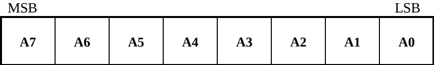
Figure 10.5. Register Address
