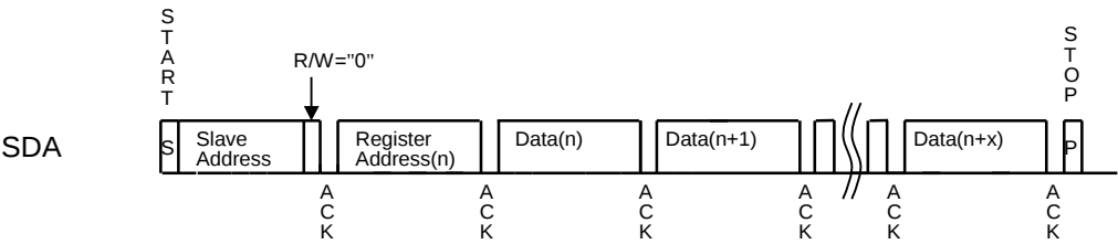
Figure 10.7. WRITE Instruction
