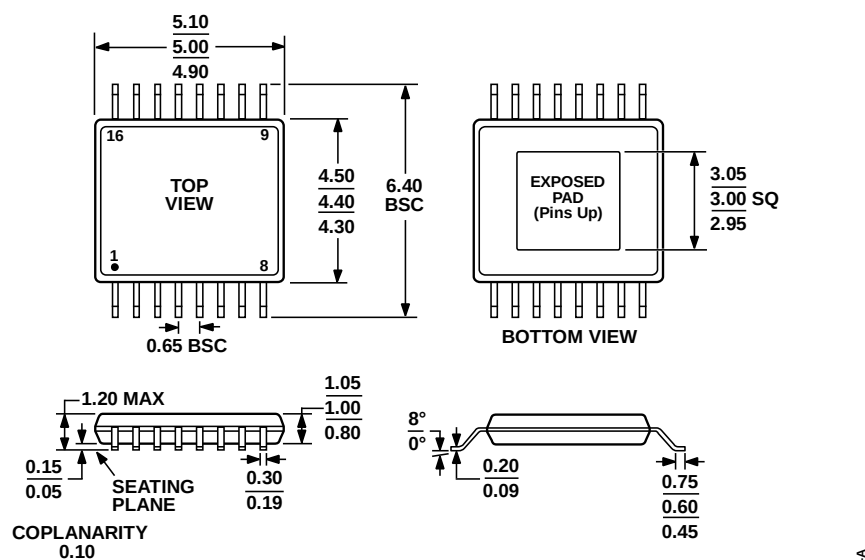
COMPLIANT TO JEDEC STANDARDS MO-153-ABT Figure 70. 16-Lead Thin Shrink Small Outline Package with Exposed Pad [TSSOP_EP] (RE-16-2) Dimensions shown in millimeters
