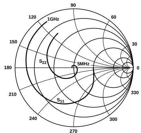
Figure 19. Input and Output Reflection Coefficients, S_{11} and S_{22} , Z_0 = 100\text{ }\Omega Differential
