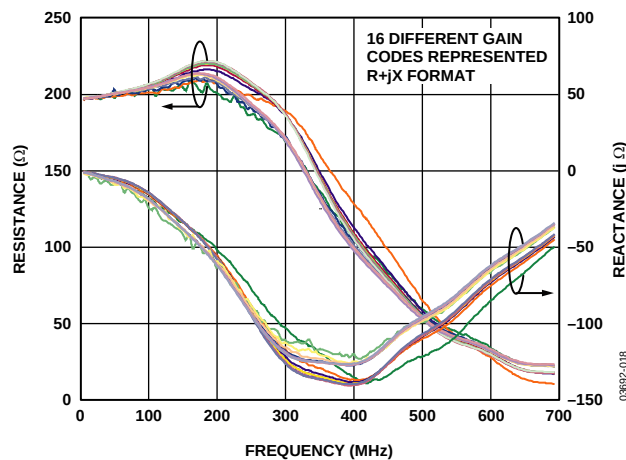
Figure 20. Input Resistance and Reactance vs. Frequency
