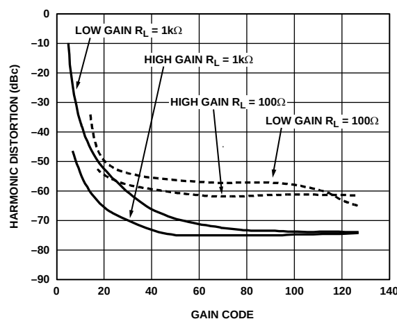
Figure 21. Third-Order Harmonic Distortion vs. Gain Code at 70 MHz, V_{OUT} = 2\text{ V p-p} Differential
