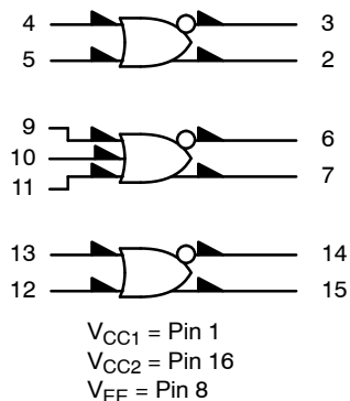
Figure 1. Logic Diagram
