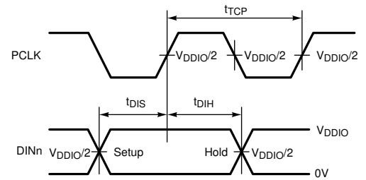
Figure 6-8. Serializer Setup/Hold Times
