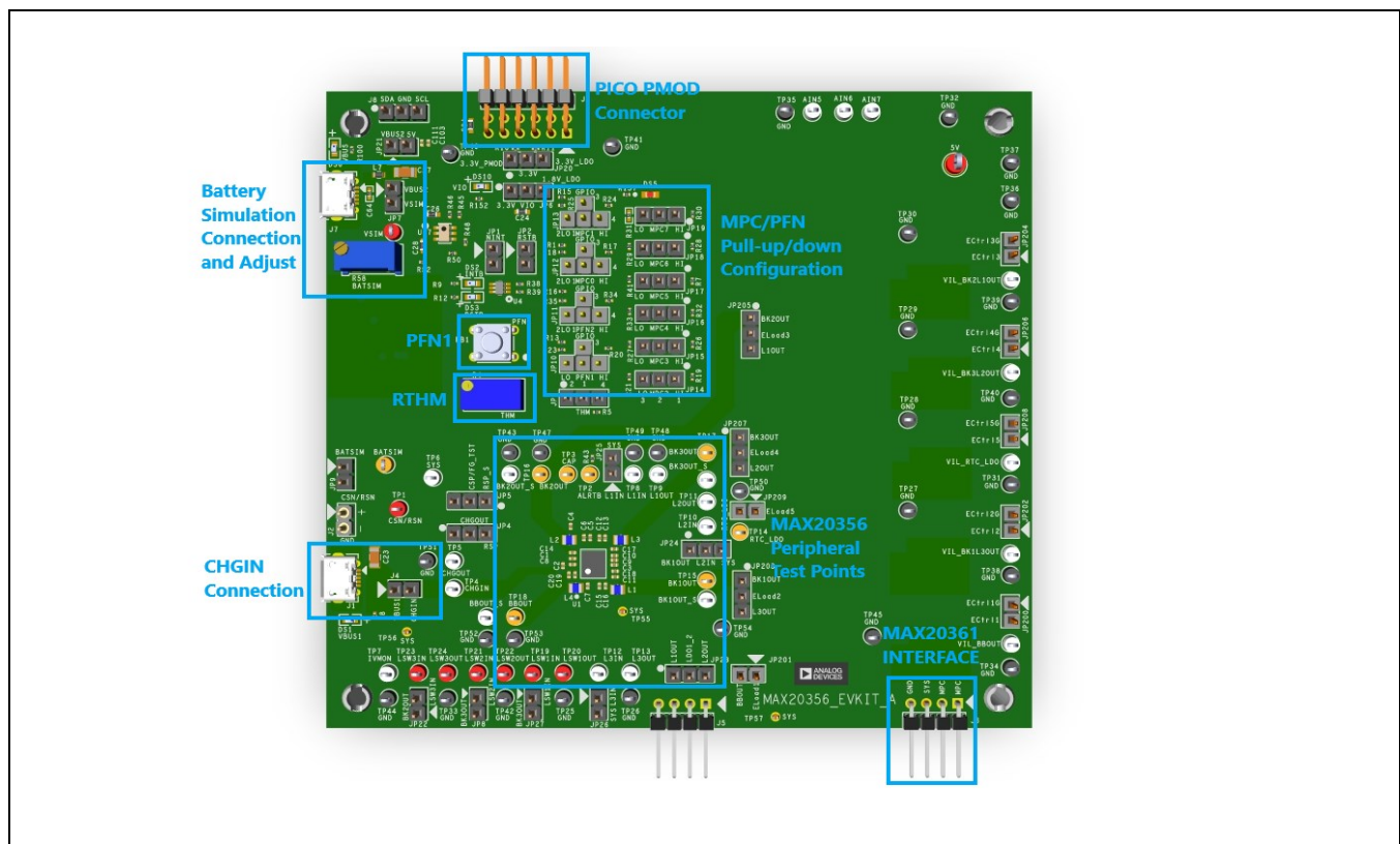
Figure 14. MAX20356 EV Kit Block Annotated Picture
