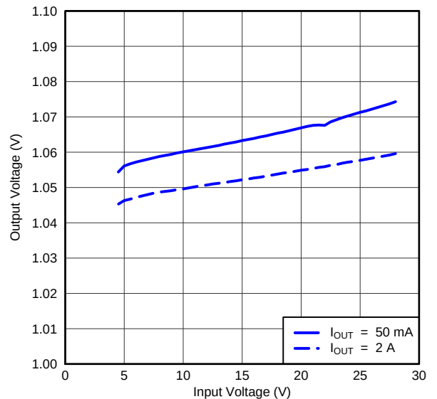
Figure 9. Line Regulation
