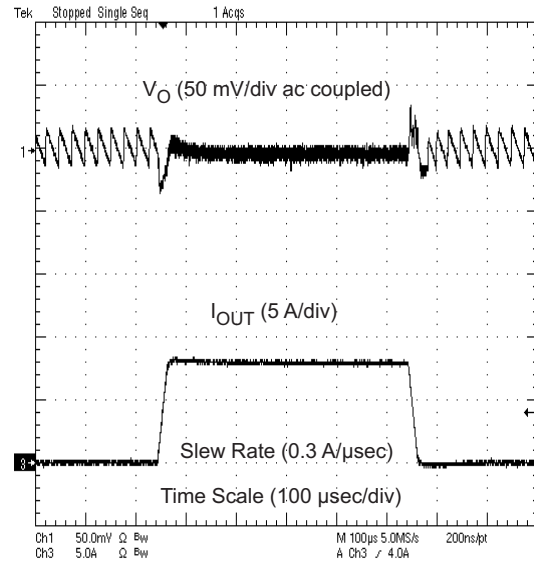
Figure 10. Transient Response
