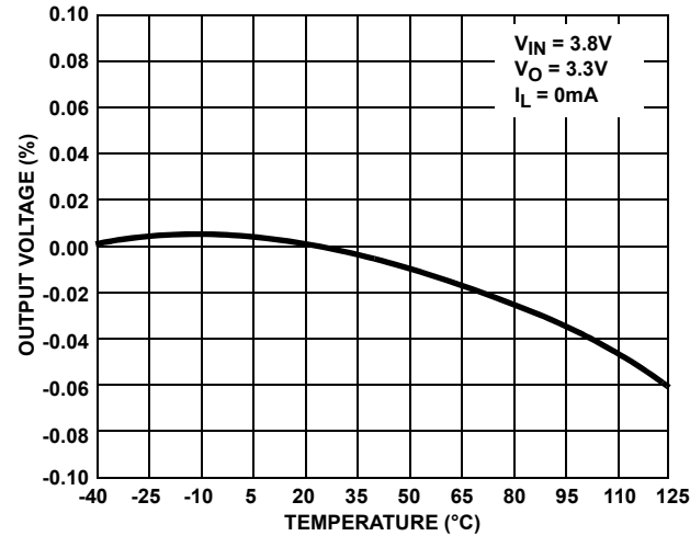
FIGURE 5. OUTPUT VOLTAGE vs TEMPERATURE
