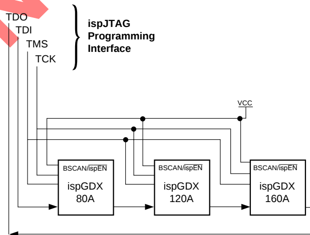
Figure 6. ispJTAG Device Programming Interface
