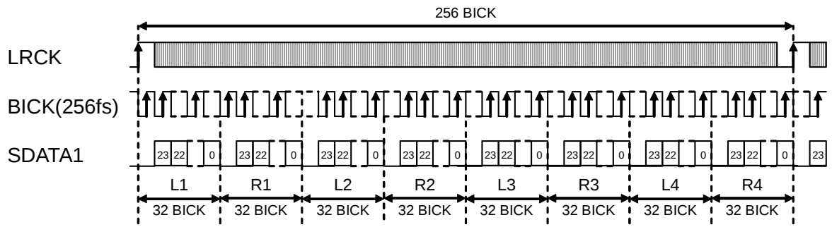
Figure 7. Mode 10 Timing
