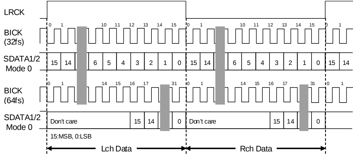
Figure 1. Mode 0 Timing
