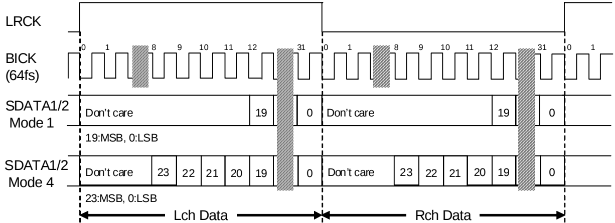
Figure 2. Mode 1/4 Timing
