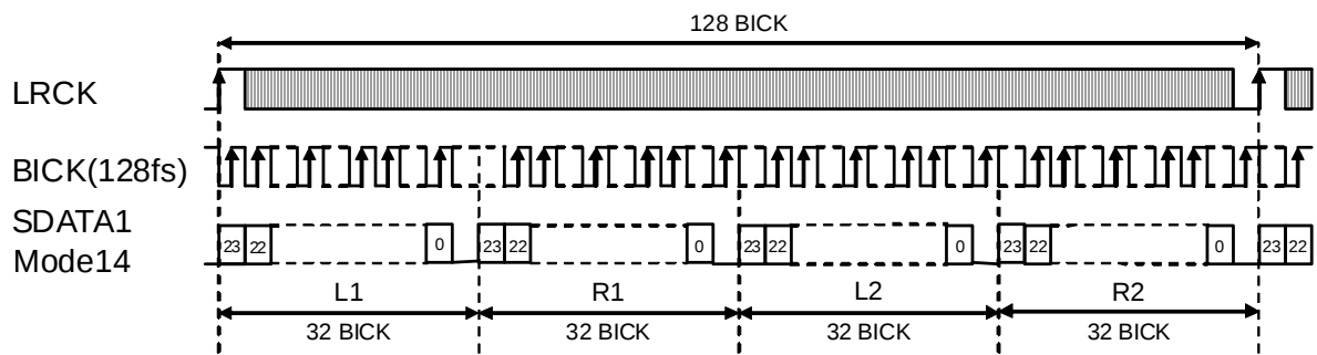
Figure 8. Mode 14 Timing
