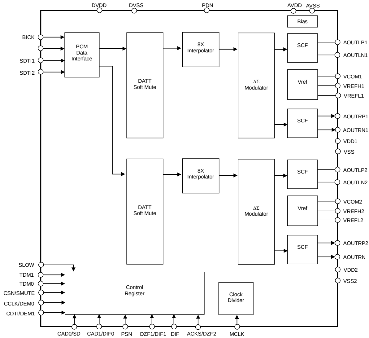
Block Diagram
