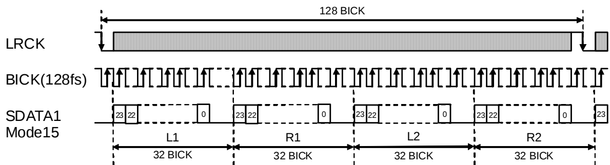
Figure 9. Mode 15/19 Timing
