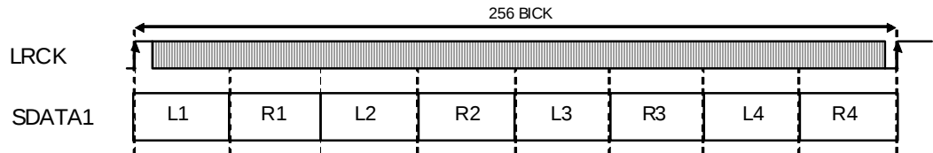
Figure 13. Data Slot in TDM256 Mode
