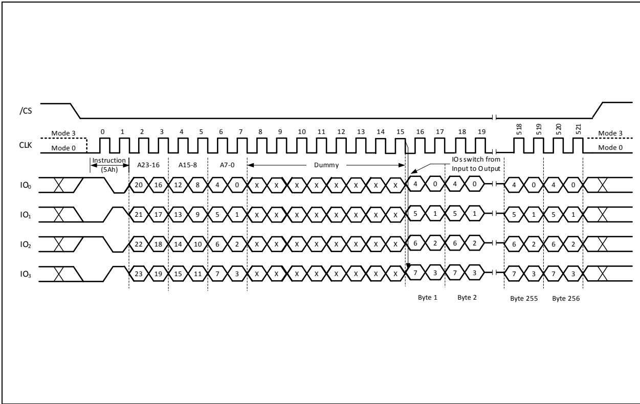
Figure 44. Read SFDP Register Instruction Sequence Diagram(QPI Mode)
