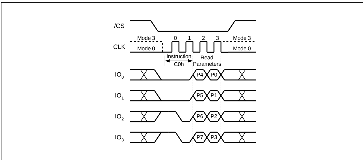
Figure 48b. Set Read Parameters Instruction (QPI Mode only)
