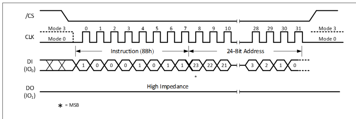
Figure 54e. Load Buffer (SPI Mode)
