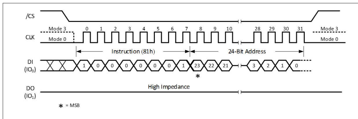
Figure 54a. Clear Buffer (SPI Mode)
