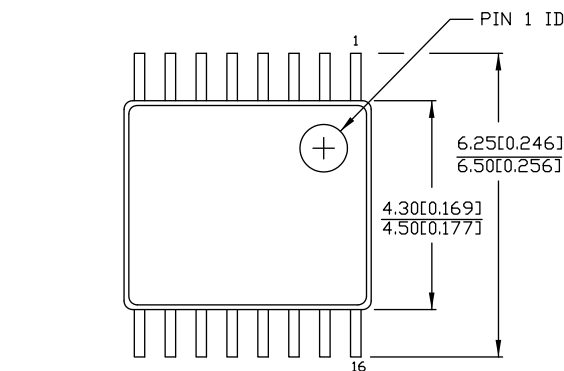
Figure 7. 16-pin TSSOP 4.40 mm Body Z16.173/ZZ16.173 Package Outline, 51-85091
