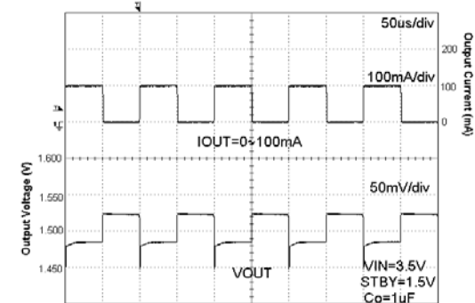
Fig. 24 Load Response Current Pulse=10 kHz
