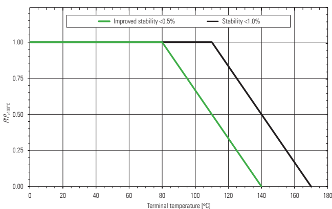
Power derating curve BVT-I-R003 / R004 / R0045 / R005 / R0068
